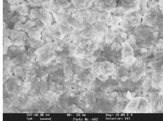
Fig. 5c. SEM image of ZnSA6 composite.
